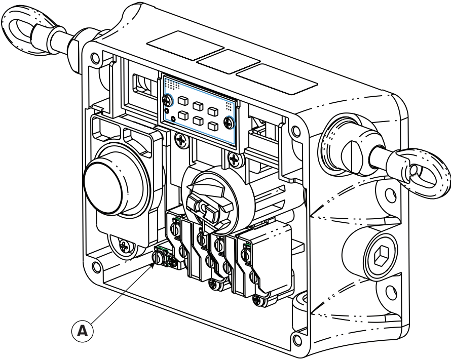
FIGURE 4. CONTACTS
