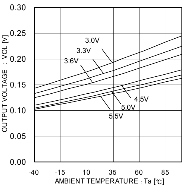
Figure 12. SEROUT low side voltage (Temperature characteristic @ ISO=4mA)
