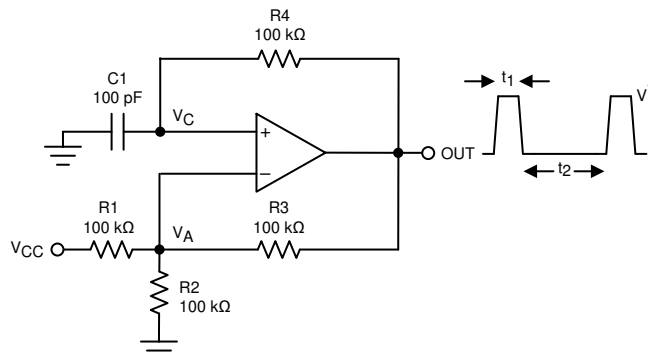
Figure 8-9. Square-Wave Oscillator
