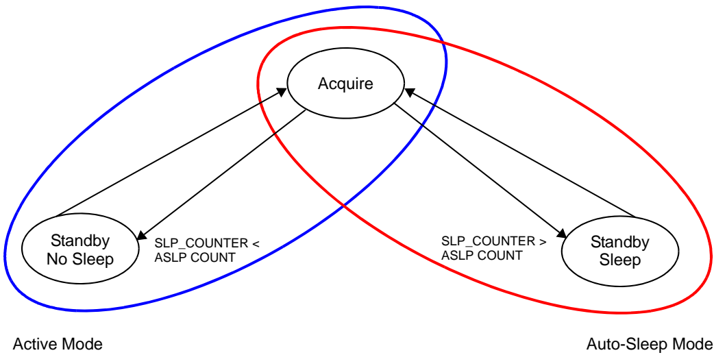
Figure 12. Auto-Sleep state transition diagram
