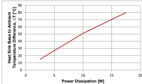
60 mm Diameter Heat Sinks
