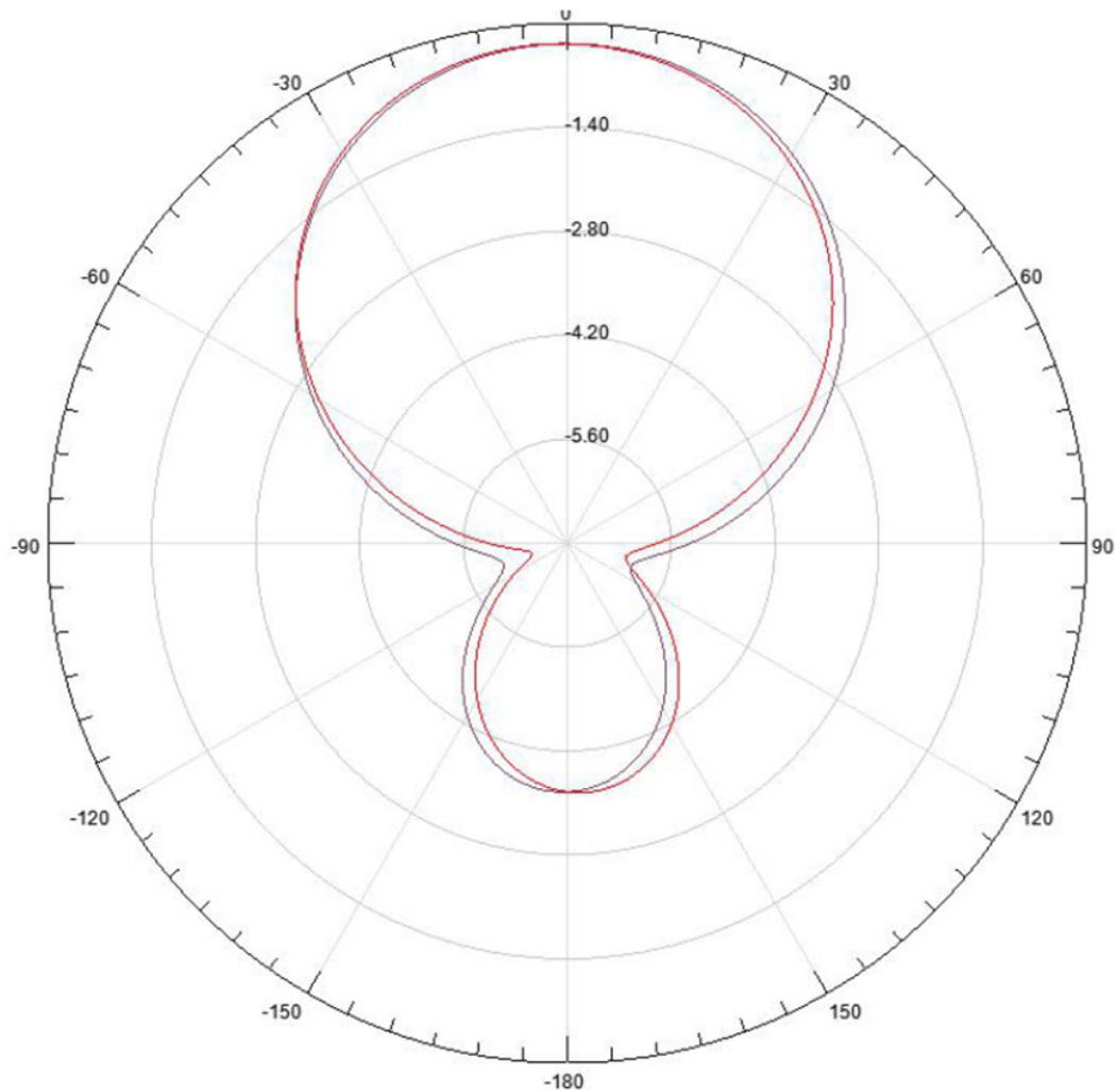
2D - Pattern YZ & XZ - Plane 1602 MHz
