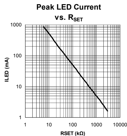
Figure 2. Peak LED Current vs. R_{SET}
