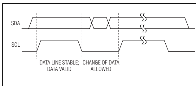
Figure 10. Bit Transfer
