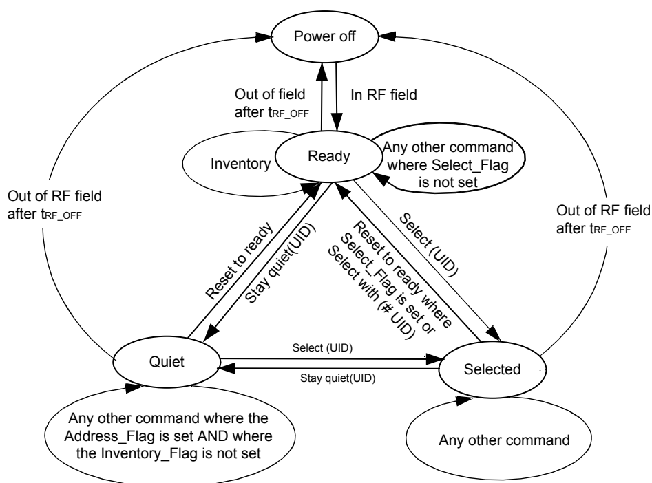
Figure 9. state transition diagram
