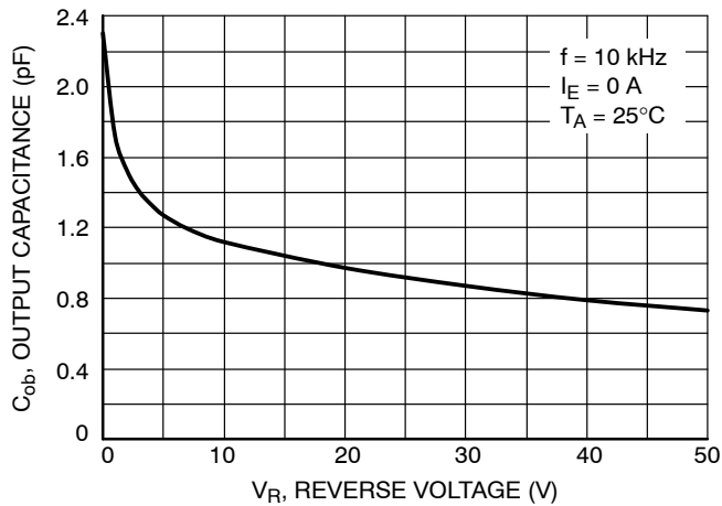
Figure 138. Output Capacitance
