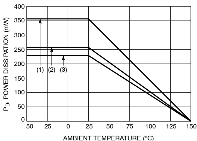
Figure 130. Derating Curve
