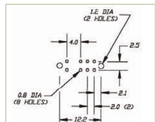
P.C. MOUNTING
