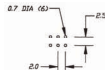
P.C. MOUNTING
