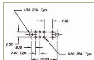
P.C. MOUNTING
