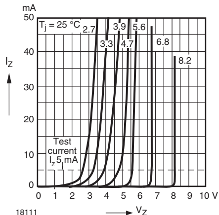
Fig. 12 - Breakdown Characteristics
