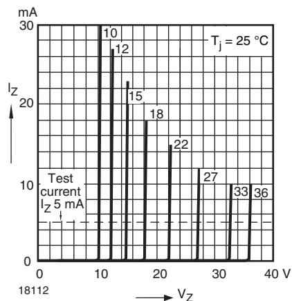
Fig. 13 - Breakdown Characteristics
