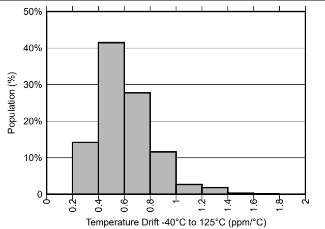
Figure 7-2. Temperature Drift Distribution
