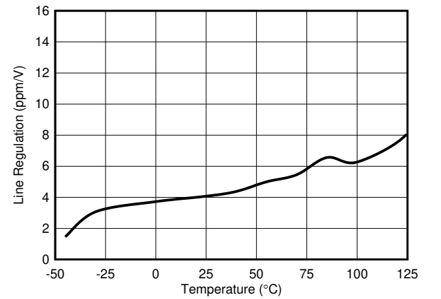
Figure 7-4. Line Regulation vs Temperature
