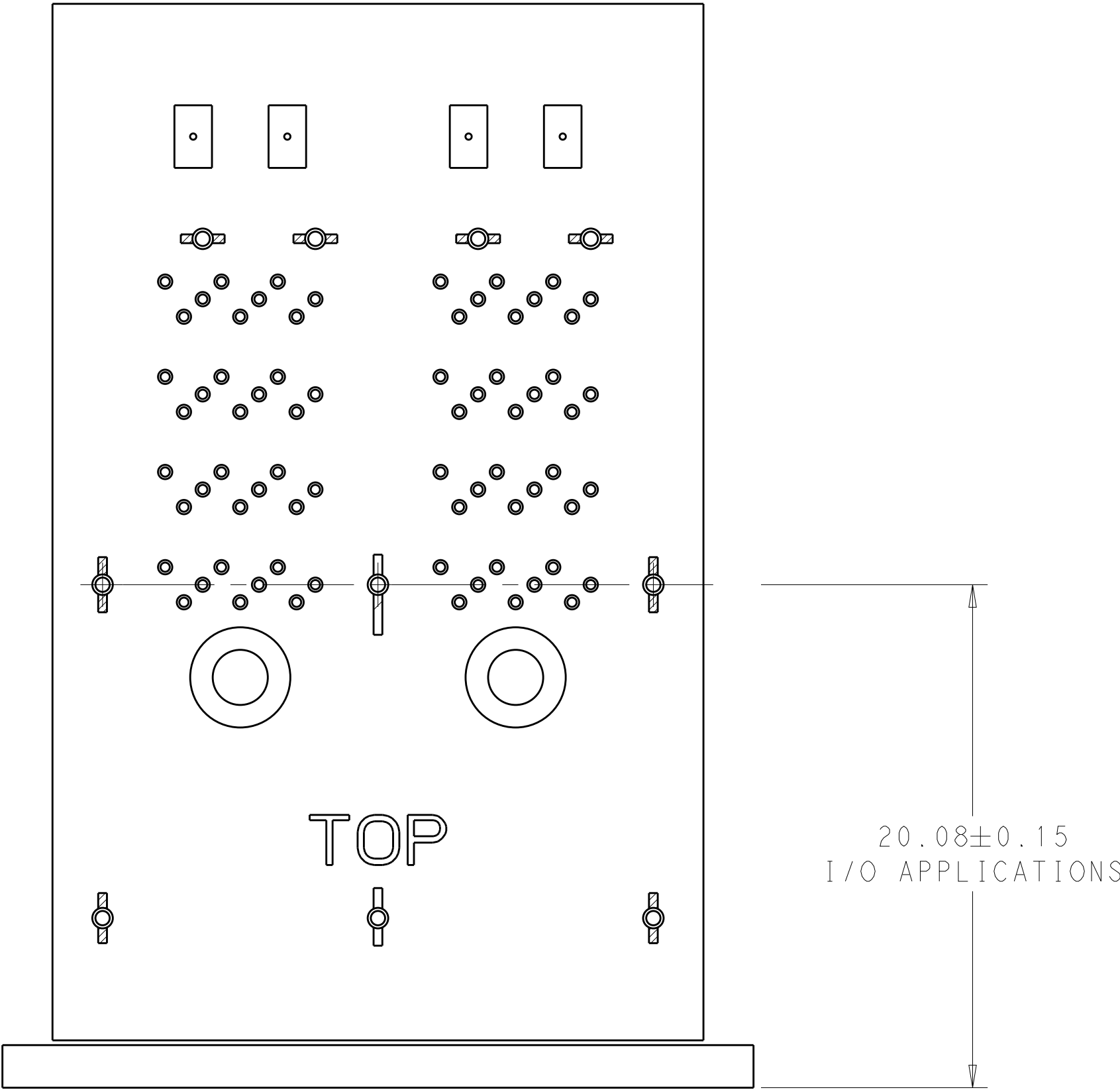
PANEL/PCB ASSEMBLY SCALE 5:1
