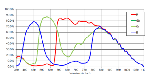
MV-CH120-60GC 量子效率
