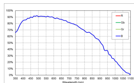
MV-CH120-60GM 量子效率
