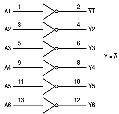
Figure 1. Logic Diagram
