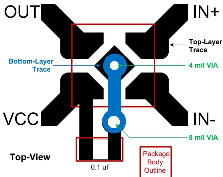
Figure 42. Layout Example
