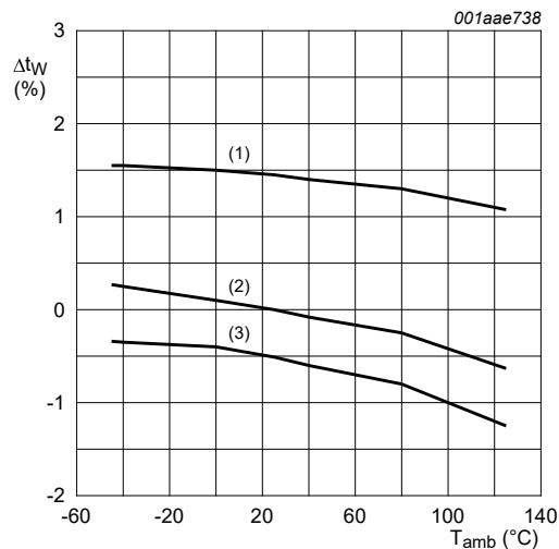
a. R_{EXT} = 100\text{ k}\Omega ; C_{EXT} = 100\text{ nF} (1) V_{DD} = 5\text{ V} (2) V_{DD} = 10\text{ V} (3) V_{DD} = 15\text{ V} \Delta t_W = 0\% at V_{DD} = 10\text{ V} and T_{amb} = 25\text{ }^\circ\text{C}
