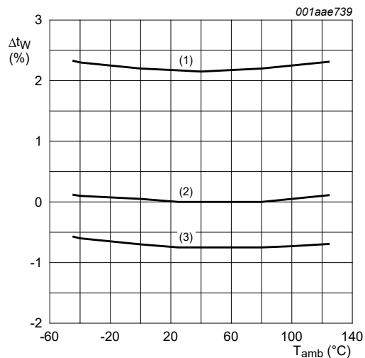
b. R_{EXT} = 100\text{ k}\Omega ; C_{EXT} = 2\text{ nF} (1) V_{DD} = 5\text{ V} (2) V_{DD} = 10\text{ V} (3) V_{DD} = 15\text{ V} \Delta t_W = 0\% at V_{DD} = 10\text{ V} and T_{amb} = 25\text{ }^\circ\text{C}
