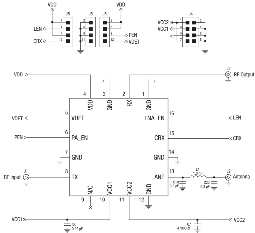
Figure 3. SKY85712-11 Application Schematic
