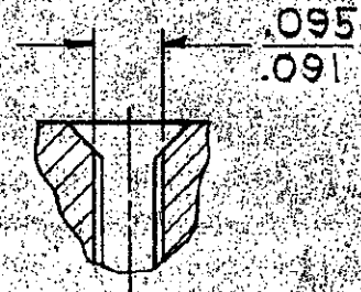
SECT. B-B
