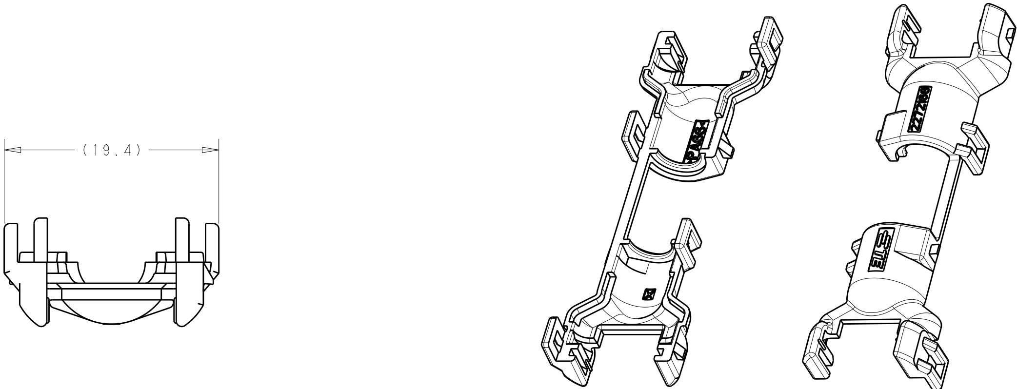
ISOMETRIC VIEWS SCALE 2:1
