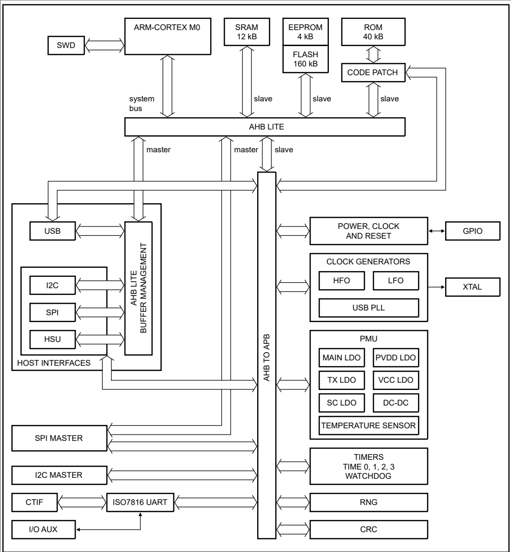
Figure 3. Block diagram
