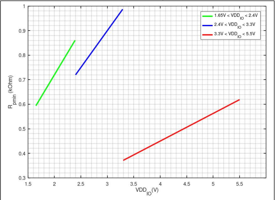
Figure 33. R_{Pmin} vs. V_{DD} , f_c = 3.4 MHz
