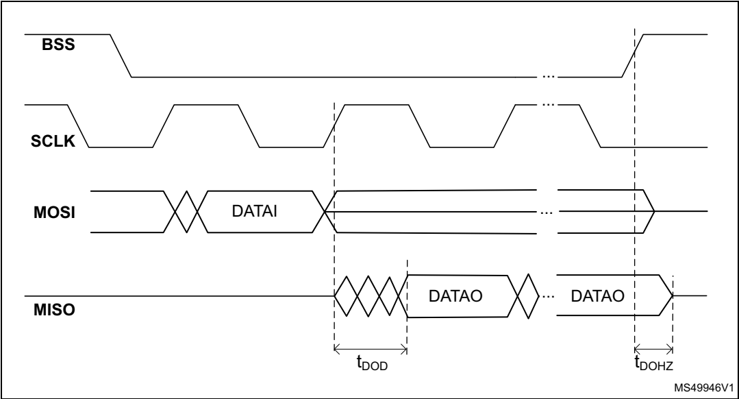
Figure 32. SPI timing diagram - Read operation
