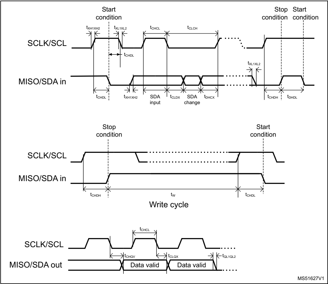
Figure 35. I2C AC waveforms
