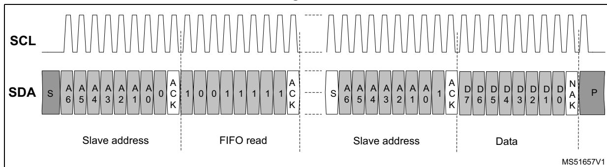
Figure 25. FIFO read
