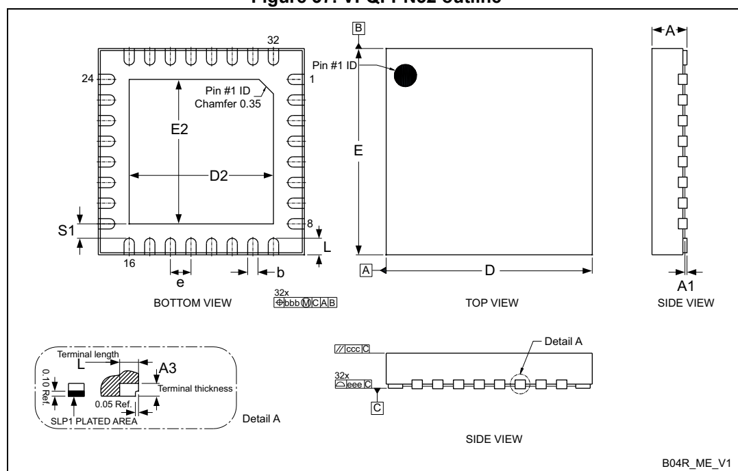
Figure 37. VFQFPN32 outline
