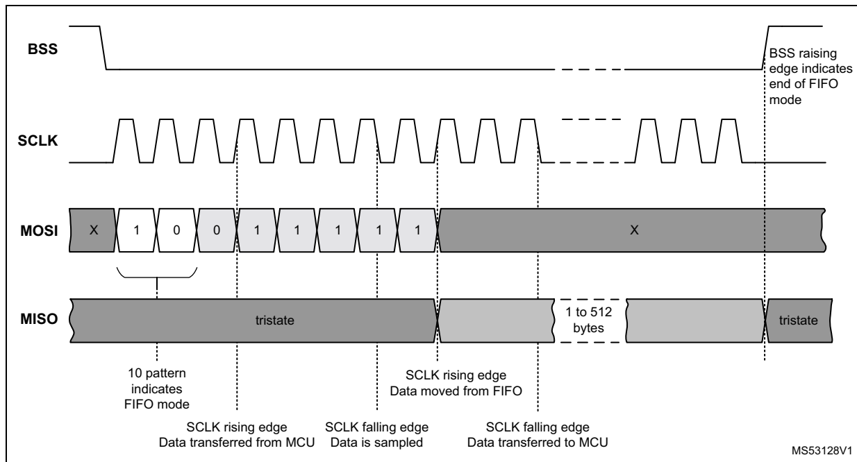
Figure 18. SPI communication: FIFO reading
