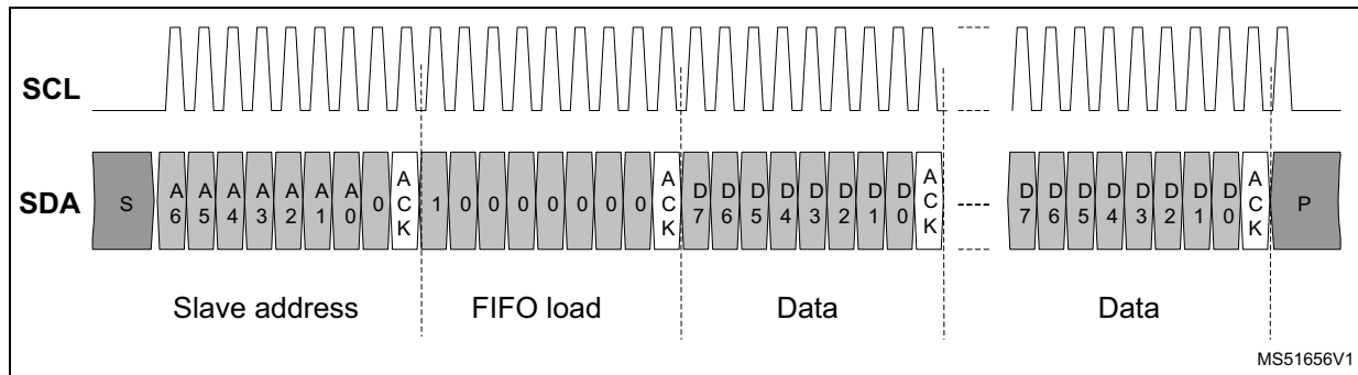
Figure 24. FIFO load
