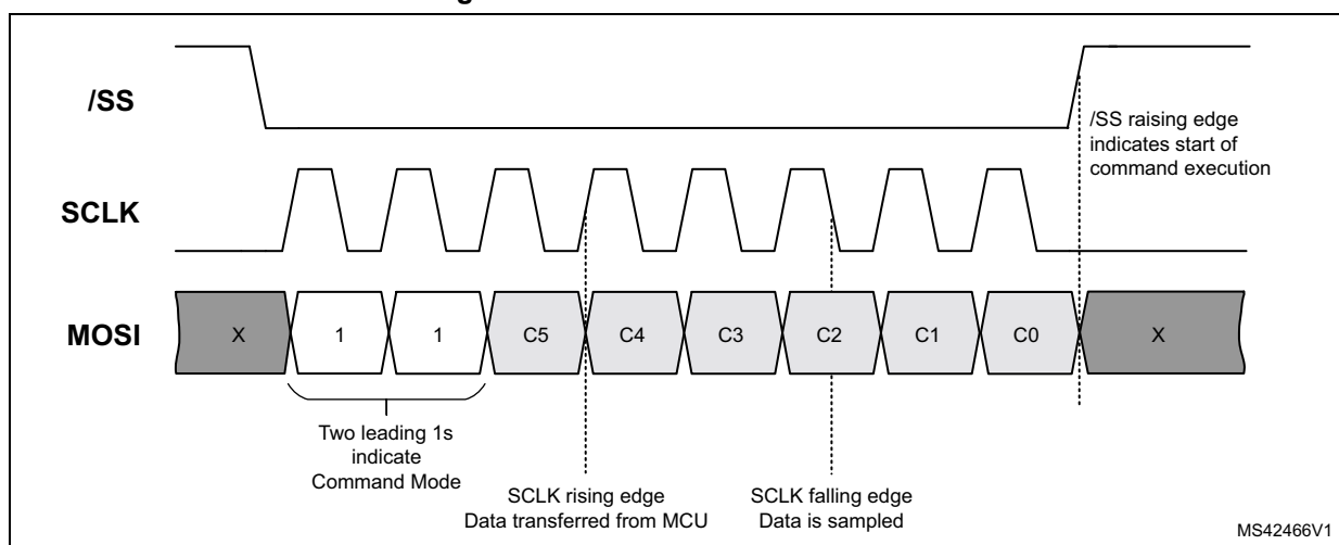
Figure 19. SPI communication: direct command
