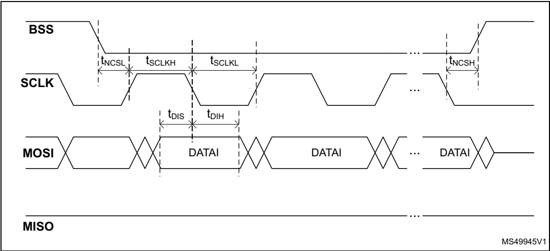
Figure 31. SPI timing diagram - General operation
