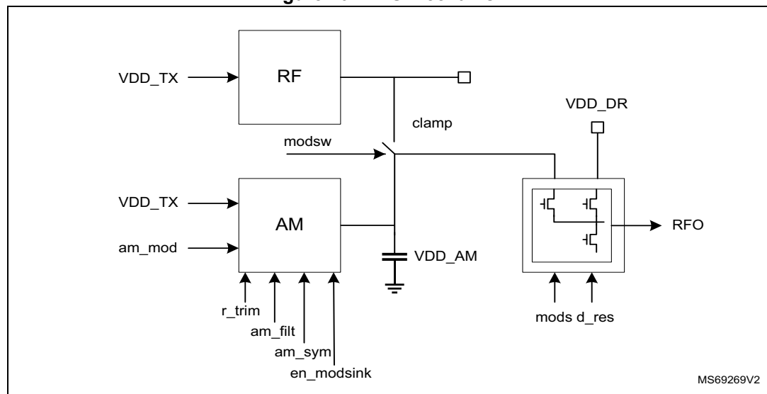
Figure 10. AWS mechanism
