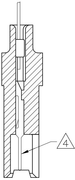
CRIMPED CONTACT FOR REF ONLY
