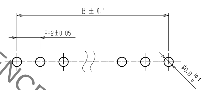
RECOMMENDED PATTERN(BOARD THICKNESS t=1.6\text{mm} )
