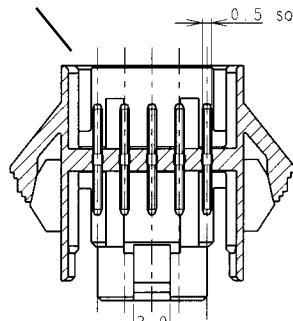
SECT B-B
