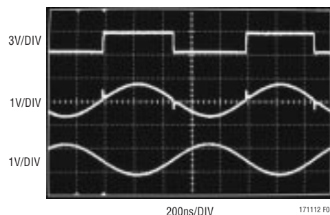
Figure 8. Oscillator Waveforms with V_S = 3V . Top is Comparator Output. Middle is Xtal Feedback to Pin 2 at LT1713 (Note the Glitches). Bottom is Buffered, Inverted and Bandpass Filtered with a Q = 5 by LT1806
